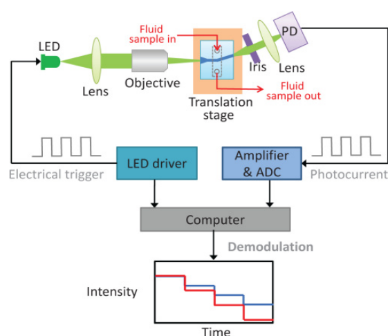
Fig. 4 Schematic of the transmission measurement system for the fabricated optofluidic waveguide refractive-index sensors.
